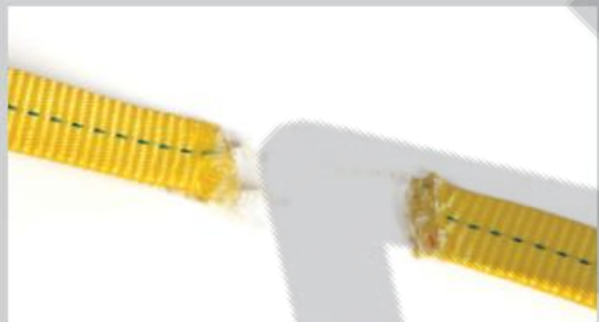
Traditional webbing lifeline (with energy absorber) failure
